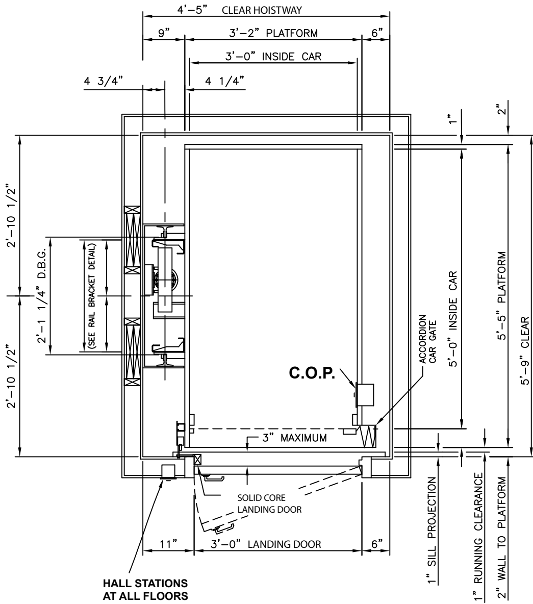
TYPICAL 3' X 5' L/H WITH LEFT HAND LANDING DOORS
